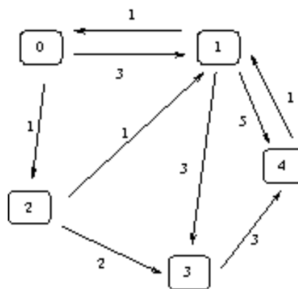
FIGURE B.16 – Chemins minimaux
